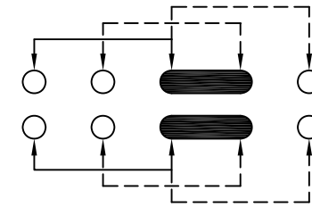
SCHEMATIC (SHORTING)
